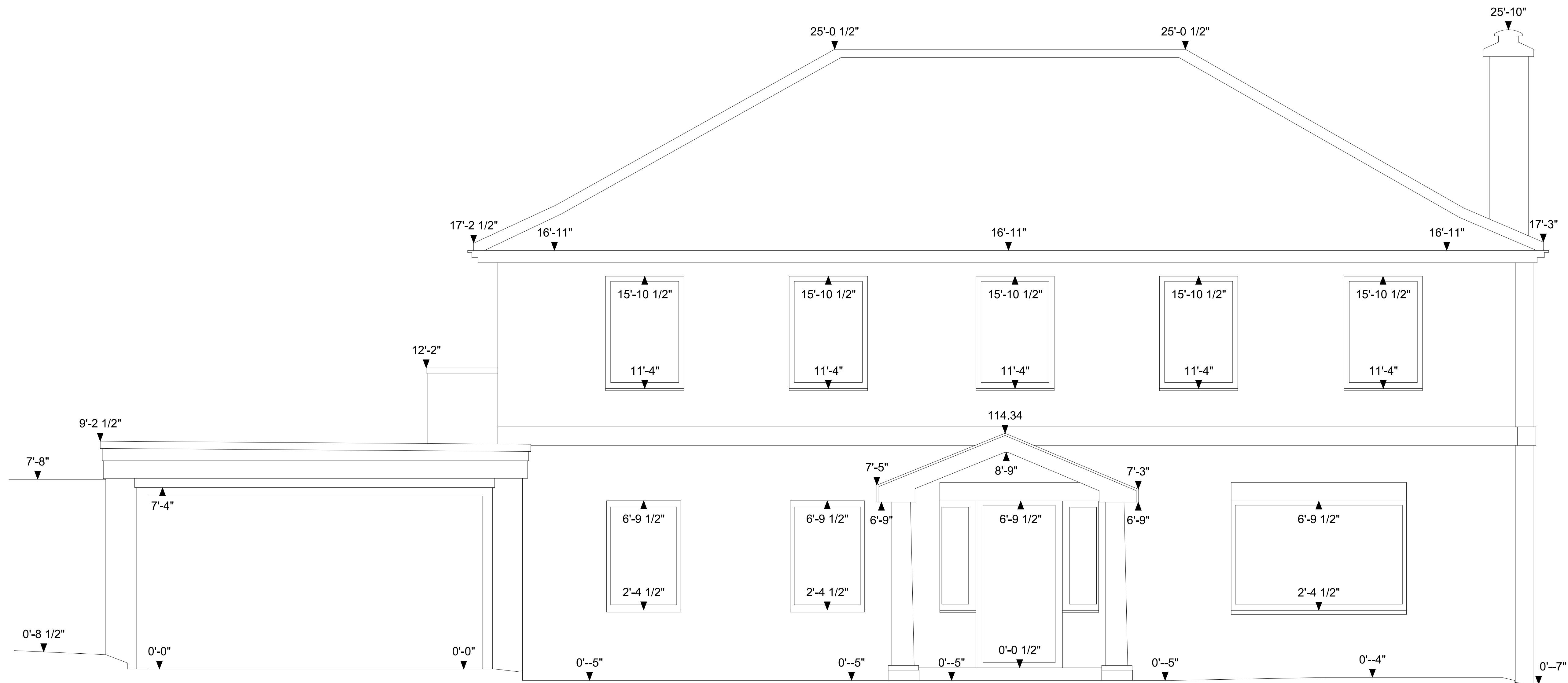
1 Elevation 1
